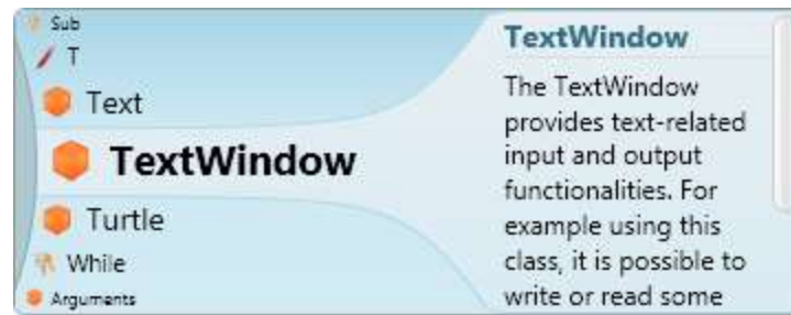
Figure 4 - Intellisense
