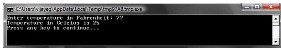
Figure 13 - Temperature Conversion
