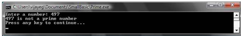
Figure 47 - Prime Check
