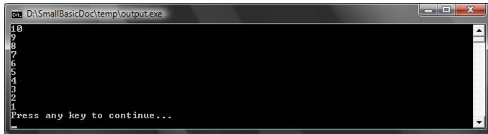
Figure 21 - Counting Backwards
