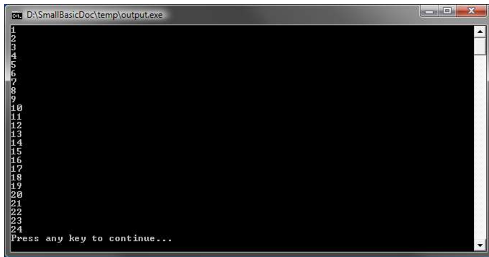
Figure 17 - Using Goto
