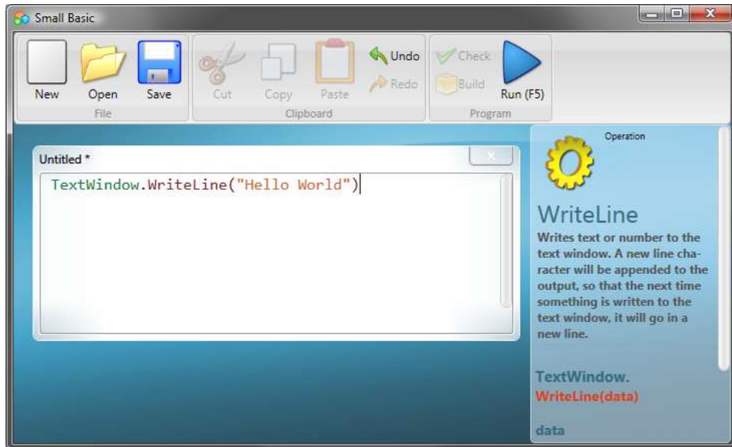
Figure 2 - First Program
