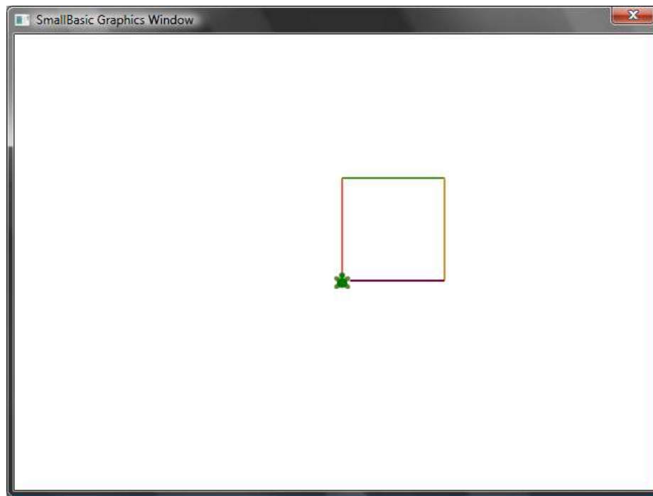
Figure 40 - Changing Colors
