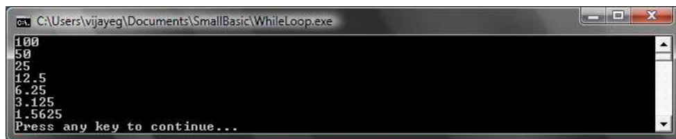
Figure 22 - Halving Loop
