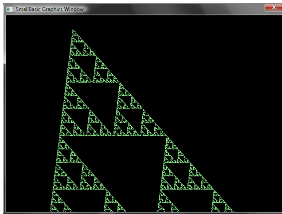
Figure 36 - Triangle Fractal
