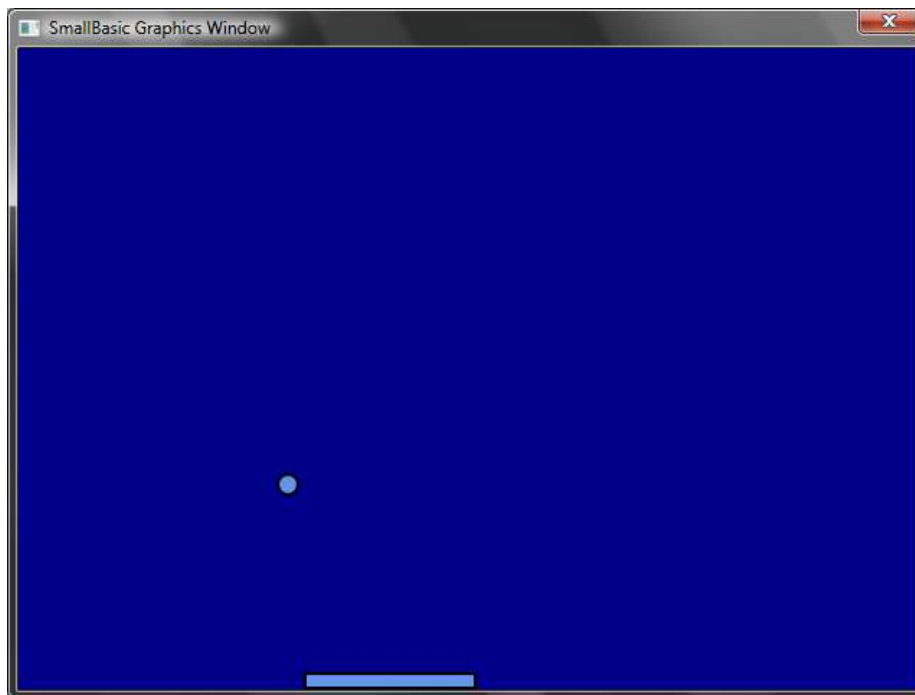
Figure 54 - Paddle Game
