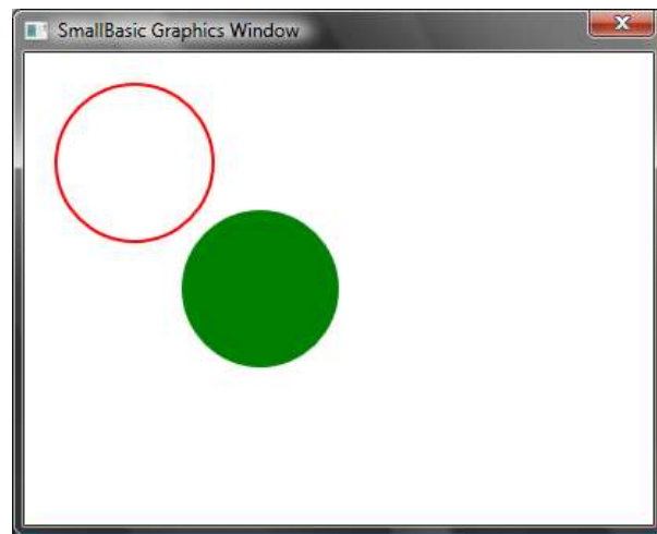
Figure 32 – Circles
