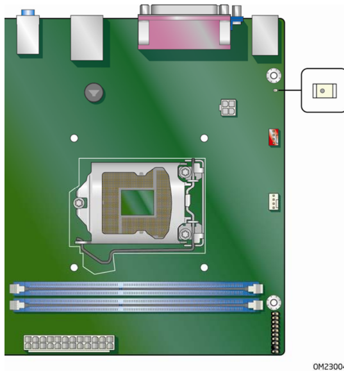
Figure 3. Location of the Standby Power Indicator
