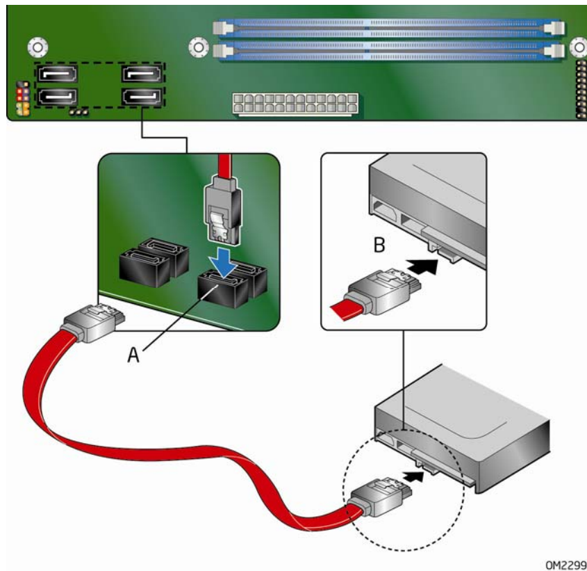
Figure 17. Connecting a Serial ATA Cable
