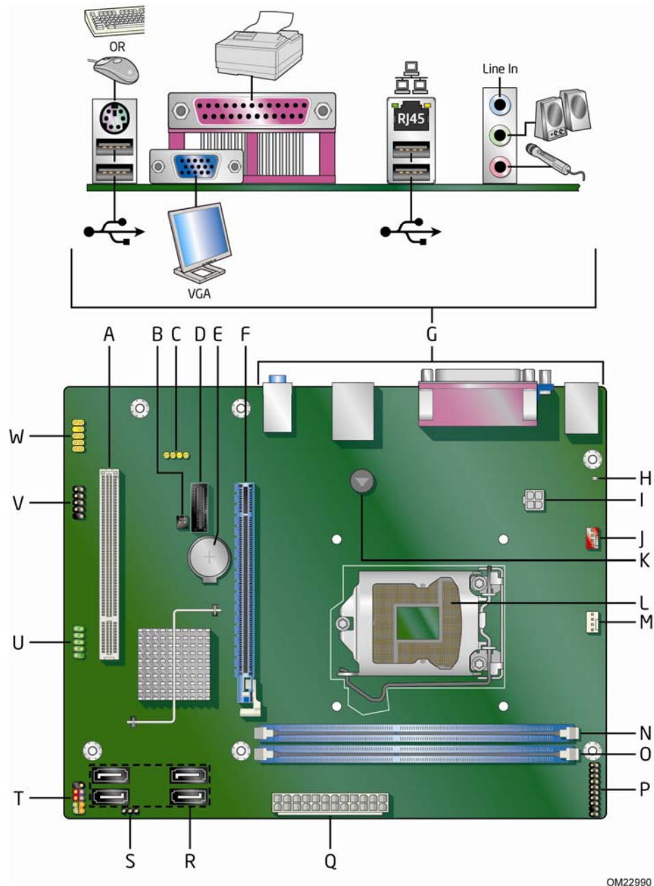
Figure 1. Intel Desktop Board DH61WW Components
