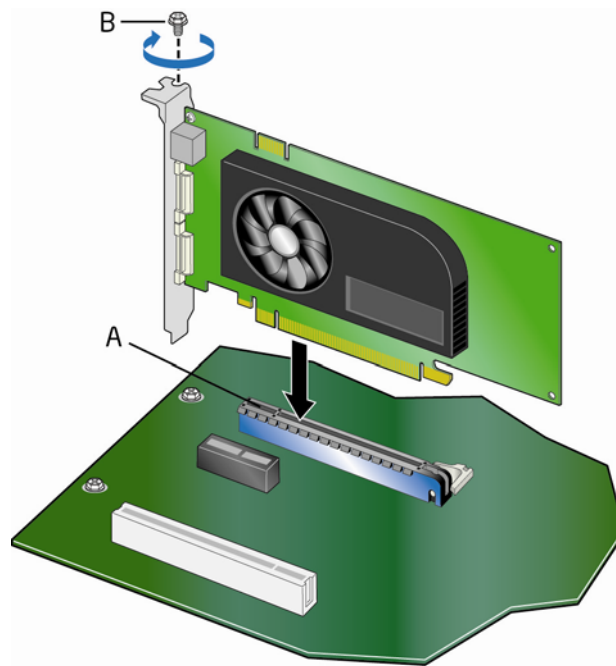
Figure 15. Installing a PCI Express x16 Graphics Card
