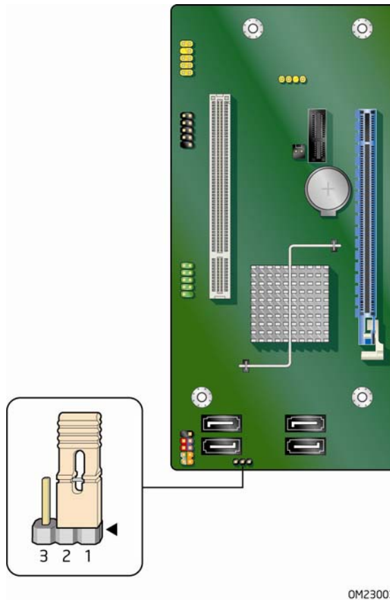
Figure 22. Location of the BIOS Configuration Jumper Block
