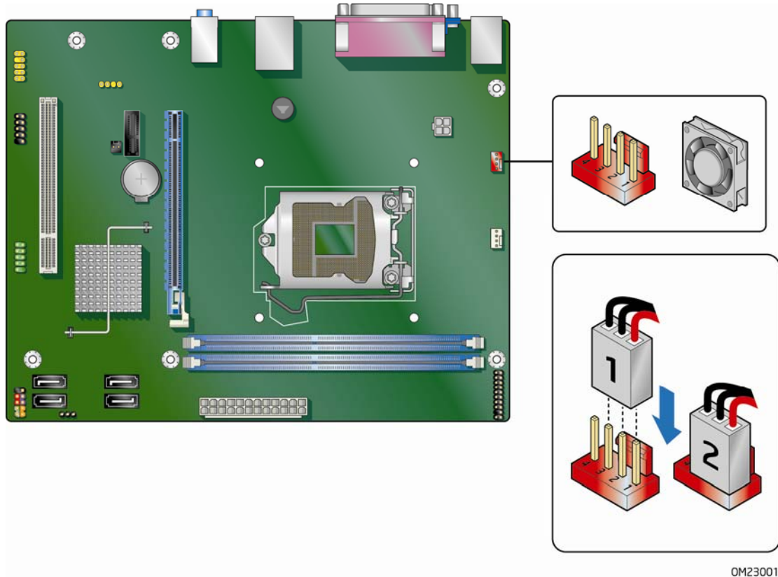
Figure 20. Location of the Chassis Fan Header
