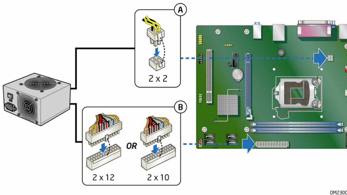
Figure 21. Connecting Power Supply Cables
