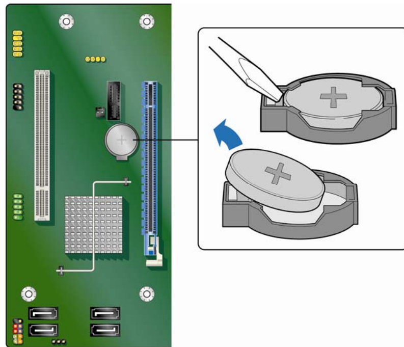
Figure 23. Removing the Battery
