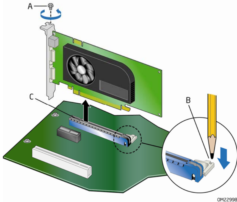
Figure 16. Removing a PCI Express x16 Graphics Card
