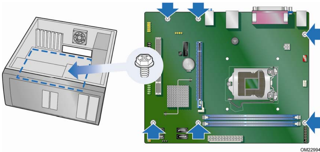
Figure 5. Intel Desktop Board DH61WW Mounting Screw Hole Locations
